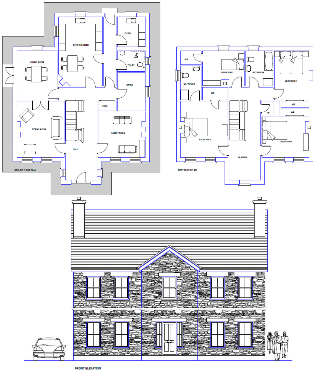
FRONT ELEVATION
