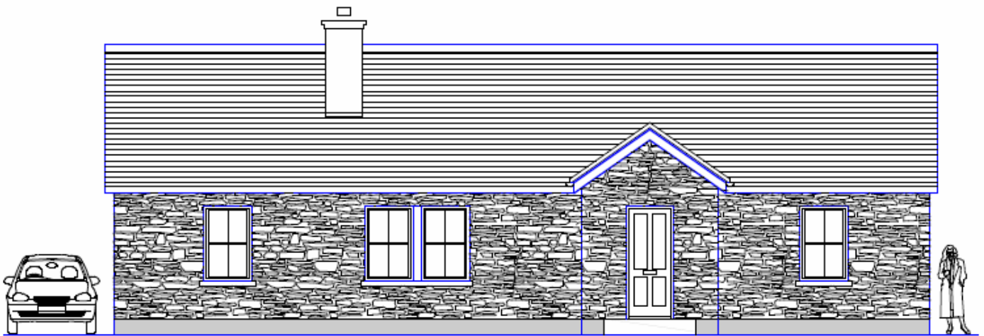
FRONT ELEVATION
