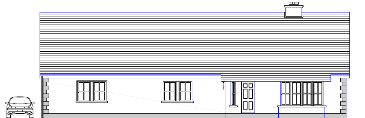
FRONT ELEVATION
